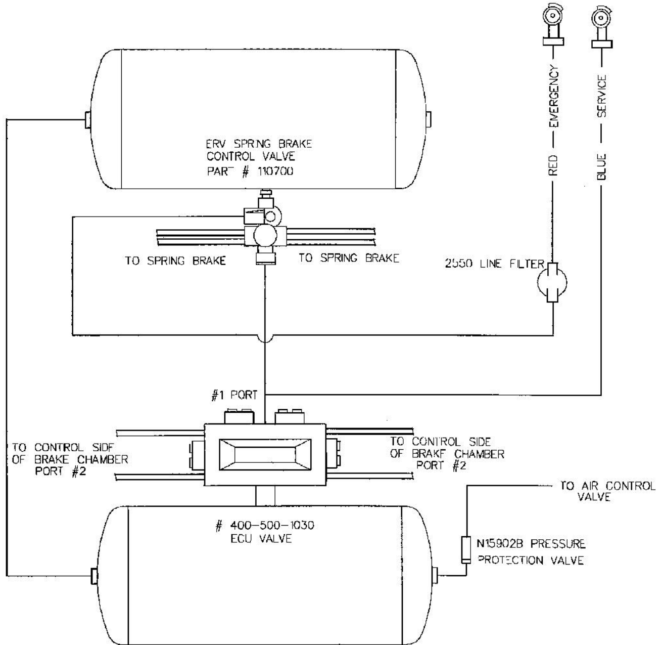
FRAMELESS AIR SYSTEM AS OF MARCH 1, 2001
